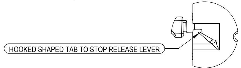
DETAIL A SCALE 2 : 3
