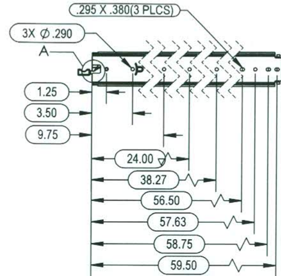
HOOKED SHAPED TAB TO STOP RELEASE LEVER
