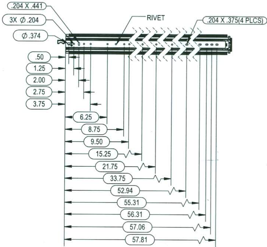
HOOKED SHAPED TAB TO STOP RELEASE LEVER
